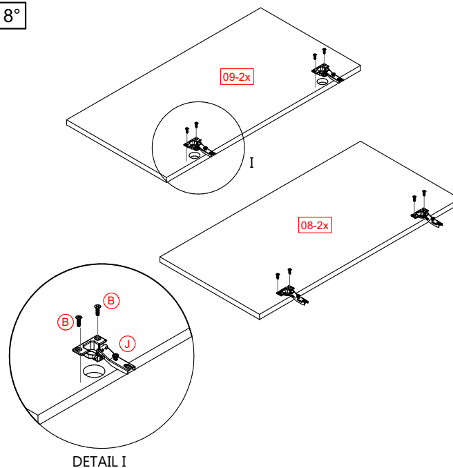
DETAIL I
