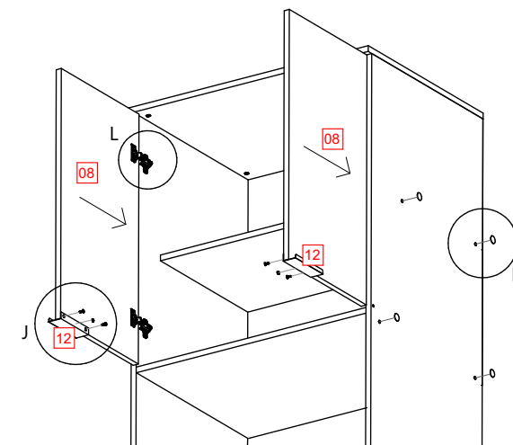
DETAIL L
