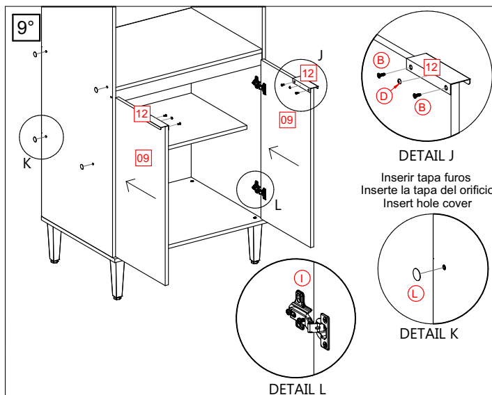
DETAIL L
